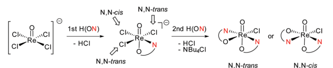
Scheme 5 Schematic representation of step-wise coordination of a bidentate ligand H(ON) (e.g. HL1a–c), with formation of N,N-trans or N,N-cis isomers. Arrows indicate point of substitution of incoming phenolate oxygen of the second H(ON) ligand and resulting stereoisomer.
