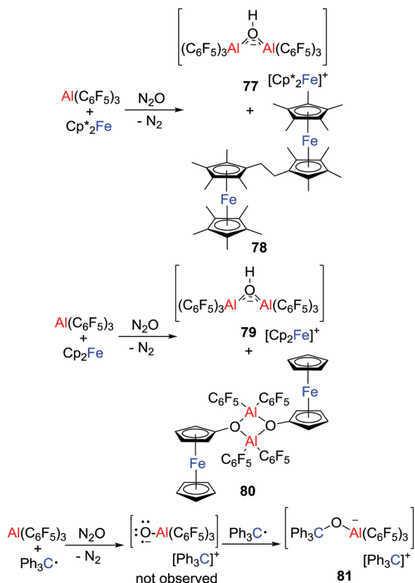
Scheme 21 Reaction of \text{Cp}^*_2\text{Fe}/\text{Al}(\text{C}_6\text{F}_5)_3 or \text{Ph}_3\text{C}^\bullet/\text{Al}(\text{C}_6\text{F}_5)_3 with \text{N}_2\text{O} .
