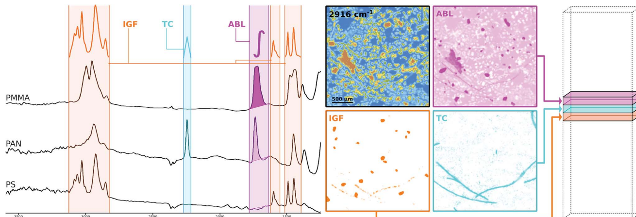
Fig. 2 Descriptor images generated using the ABL, TC and IGF descriptors. The spectra (left) correspond to three types of common polymers. By using the stated spectral descriptors on certain ranges of the hypercube the corresponding descriptor images (middle) can be computed which are then reassembled as a descriptor cube of reduced dimensionality and improved data quality (right).
