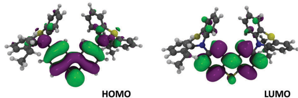
Fig. 4 Molecular orbitals, HOMO and LUMO of DPTZ-DBT (equatorial) and DPTZ- i Pr-DBT (axial) forms at DFT (M062X)/Def2SVP level of theory.
