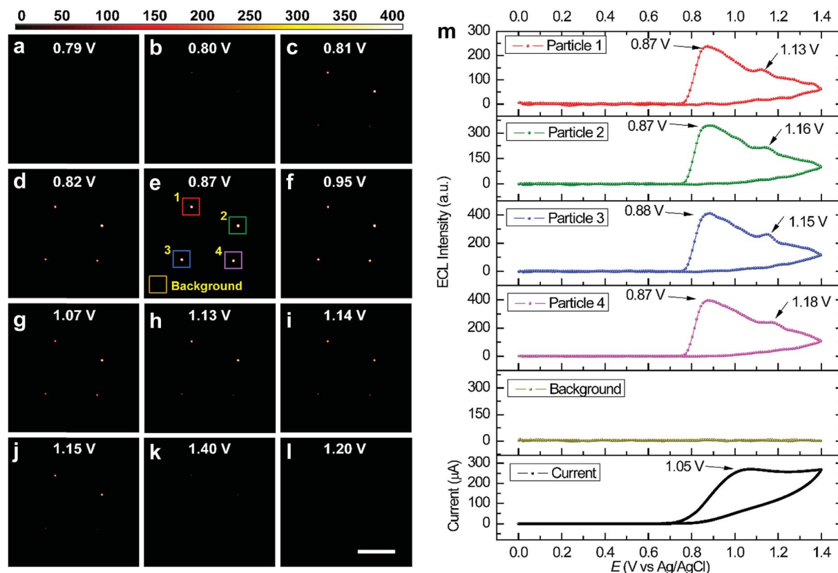
Fig. 2 (a–l) Successive ECL snapshots of four RuDSNs during a potential cycle. Scale bars (white), 30 \mu m. (m) ECL intensity of four nanoparticles and blank area in (e) as a function of electrode potential and the corresponding CV curve of the GC electrode (black line) recorded by the potentiostat. The potential was cyclically scanned from 0 to 1.4 V at a scan rate of 20 \text{mV s}^{-1} in 200 mM PBS buffer containing 100 mM TPA. The exposure time of EMCCD was 500 ms.
