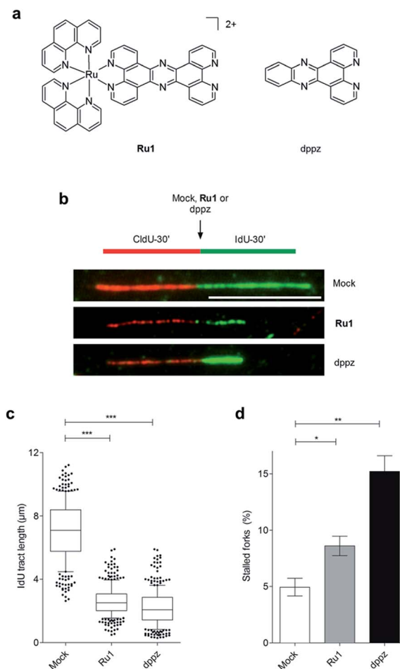
Fig. 1 (a) Structures of Ru1 and dppz. Ru1 was used as the chloride salt and as a mixture of A and A' enantiomers. (b) Representative images of DNA replication fibres in OE21 oesophageal cancer cells. CldU (first pulse, 30 min) incorporation is shown in red, incorporated IdU (second pulse, 30 min) in green. The second nucleotide (IdU) was either mock-treated or incubated in the presence of Ru1 or dppz to determine impact on DNA replication fork progression. Scale bar = 10 \mu\text{m} . (c) Quantification of IdU-labelled tract length in the presence of Ru1 (21 \mu\text{M} ) or dppz (7 \mu\text{M} ). Tract length was determined for >100 forks per condition. Whisker box plots show mean values and data within the 10–90 percentile. (d) Quantification of completely stalled forks (i.e. CldU tract only) for Ru1 or dppz treatment as in (b). Fork stalling was quantified for >300 forks per condition and experiment. The experiment was repeated three times. Data were analysed using unpaired two-tailed t test (* P < 0.1 , ** P < 0.01 , *** P < 0.005 ).
