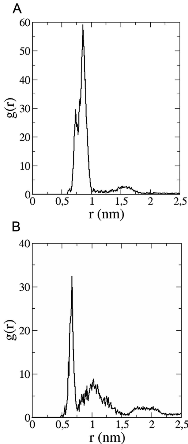
Fig. 8 (A) Radial distribution function versus distance of 5R residue (Aβ 42 ) between centres of mass of residue and fullerene trisadduct. (B) Radial distribution function as a function of the distance between the centre of mass of 1D residue and the two oxygen atoms in the COO-group.
