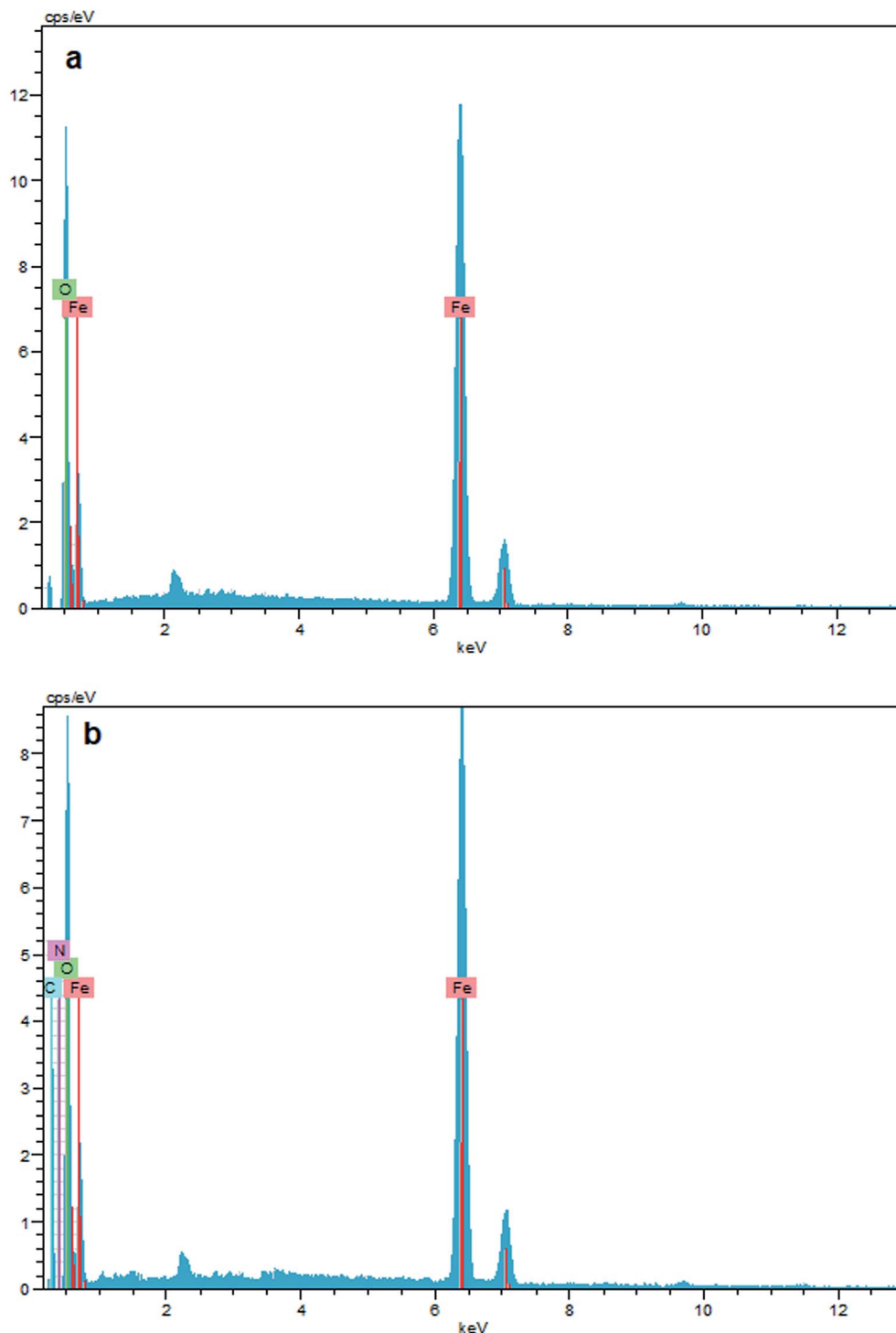
Fig. 10 EDX result of (a) \text{Fe}_3\text{O}_4 , and (b) \text{Fe}_3\text{O}_4 -chitosan particles.
