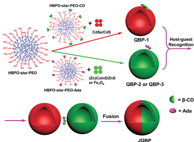
Scheme 1 The self-assembly pathway towards Janus vesicles. HBPO-star-PEO denotes an amphiphilic hyperbranched multi-arm copolymer with a hydrophobic hyperbranched poly(3-ethyl-3-oxetanemethanol) (HBPO, in blue) core and hydrophilic poly(ethylene oxide) (PEO, in red) arms; HBPO-star-PEO-CD represents \beta -cyclodextrin functionalized HBPO-star-PEO and HBPO-star-PEO-Ada expresses adamantane-modified HBPO-star-PEO.
