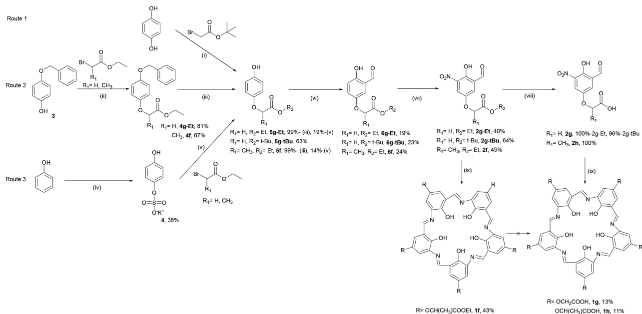
Scheme 1 Syntheses of ester/carboxylic acid campestarenes ( 1f–1h ): (i) NaOH, dioxane/ \text{H}_2\text{O} , 3 h, then HCl; (ii) \text{K}_2\text{CO}_3 , acetone, reflux, 3 h, then HCl; (iii) \text{Pd/C} , \text{H}_2 , EtOH, 12 h; (iv) \text{K}_2\text{S}_2\text{O}_8 , NaOH, \text{H}_2\text{O} , 24 h, then HCl; (v) \text{K}_2\text{CO}_3 , EtOH, reflux 6 h, then AcOH, reflux, 2 h; (vi) \text{Et}_3\text{N} , \text{MgCl}_2 , \text{CH}_2\text{O} , MeCN, reflux, 24 h, then HCl; (vii) \text{HNO}_3 , AcOH, 2 h; (viii) \text{R}_2 = \text{Et} , NaOH, MeOH/ \text{H}_2\text{O} , 12 h, then HCl or \text{R}_2 = t\text{-Bu} , TFA/DCM, 12 h; (ix) \text{Na}_2\text{S}_2\text{O}_4 , EtOH/ \text{H}_2\text{O} , reflux, 2 h.
