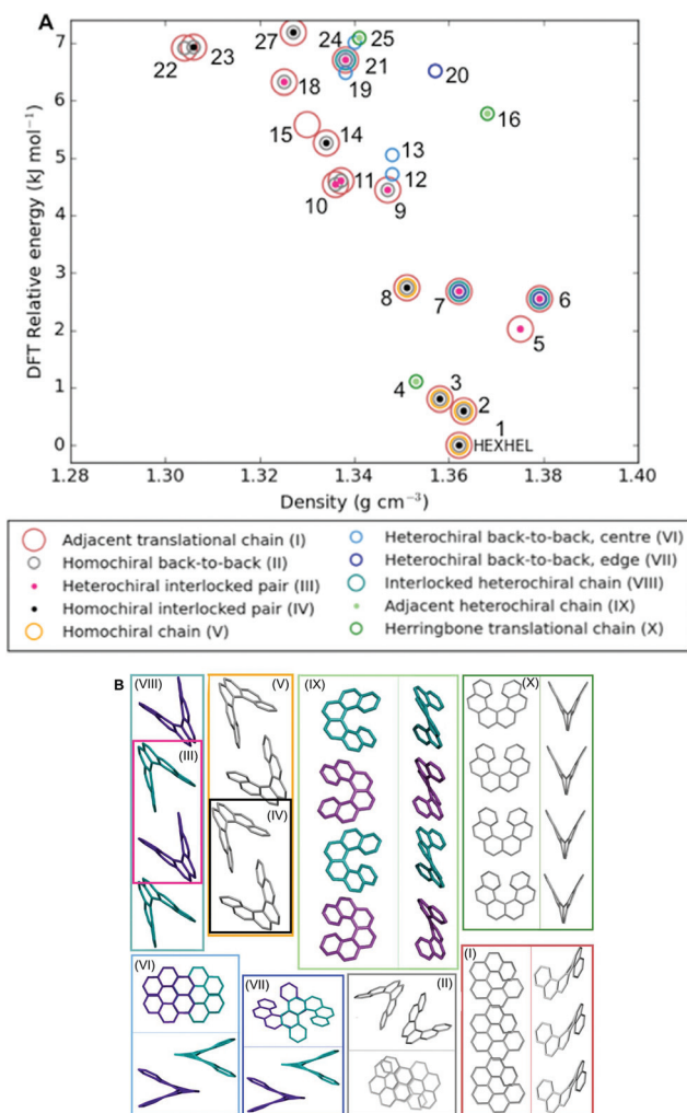
Fig. 5 (a) Lattice energy landscape labelled according to which molecular substructures they contain. Substructures are ordered by decreasing frequency. Note, two predicted structures ( 17 and 26 ) do not appear on the plot as they contain none of these substructures, for their positions, refer back to Fig. 3; (b) the molecular substructures, with surrounding boxes coloured and labelled as per (a). Where necessary, two perpendicular views of the same substructure are shown within the box, divided by a line. Helicene molecules within homochiral substructures are shown grey and within heterochiral substructures opposite enantiomers are shown purple and cyan; no hydrogens are shown. Table S1† gives the substructures found in each of the 27 structures.
