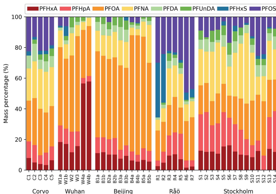
Fig. 2 Homologue pattern of PFAAs displayed as percentage by weight in precipitation sampled on Corvo (C), in Wuhan (W), in Beijing (B), on Rào (R) and in Stockholm (S). Each data point represents an individual sample. PFOA and PFOS concentrations are expressed as the sum of branched and linear isomers. Concentrations below the MDL are not displayed. PFHxA was not quantified in sample S12 due to interference of the matrix.
