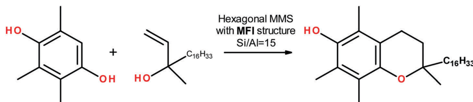
Scheme 3 Annulation of trimethylhydroquinone with isophitol yielding vitamin E.
