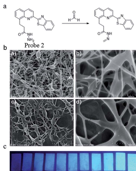
Fig. 3 (a) FA sensing mechanism of probe; (b) SEM images of polyvinyl alcohol blending probe 2 electrospun nanofibers. (a) PVA (2 μm), (b) PVA (500 nm), (c) 1 and PVA (2 μm), and (d) 1 and PVA (500 nm) and (c) photographs of probe 1 ( 2.96 \times 10^{-2} wt%) as electrospinning test strip for the detection of formaldehyde at various concentrations (from left to right: 0 M, 0.01 M, 0.05 M, 0.1 M, 0.2 M, 0.7 M, 1 M, 2 M, 3 M, 5 M, 7 M, 10 M) in water (this figure has been reproduced from ref. 51 with permission from Elsevier).
