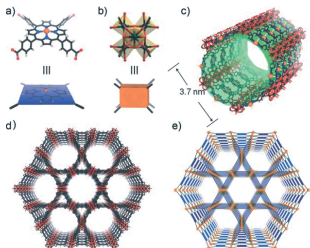
Fig. 1 The crystal structure and underlying network topology of PCN-222(Fe). The Fe-L 1 (a; blue square) is connected to four 8-connected Zr 6 clusters (b; light orange cuboid), generating a 3D network with Kagome-like topology (d, e) and large 1D channels (c; green pillar). Zr: black spheres, C: gray, O: red, N: blue, and Fe: orange. [Reprinted with permission from ref. 56. Copyright 2012, Wiley-VCH Verlag GmbH & Co. KGaA, Weinheim.]
