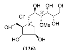
K_i = 7\text{nm} for ctSI K_i = 35\text{nm} for ntSI K_i = 500\text{nm} for ntMGAM K_i = 60\text{nm} for ctMGAM-N2 K_i = 55\text{nm} for ctMGAM-N20
