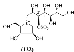
IC 50 = >236μM for Maltase IC 50 = >236μM for Sucrase IC 50 = 9μM for Isomaltase
