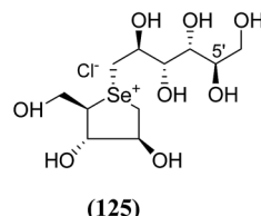
K_i = 19\text{nm} for ctSI K_i = 10\text{nm} for ntSI K_i = 25\text{nm} for ntMGAM K_i = \text{NOI} for ctMGAM-N2 K_i = 41\text{nm} for ctMGAM-N20
