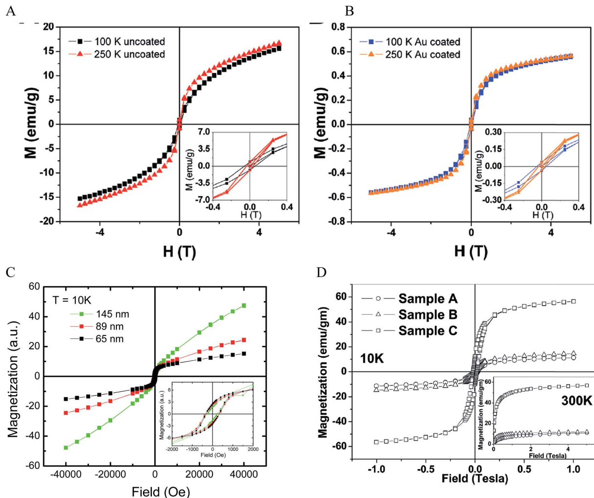
Fig. 6 Magnetic properties of IO–Au core–shell NPs. (A and B) Magnetization as a function of applied field at 100 K and 250 K for uncoated and Au coated tetracubic IO NPs. Reprinted with permission from ref. 69. Copyright (2009) American Chemical Society. (C) Magnetization as a function of applied field at 10 K for IO–Au core–shell nanopopcorns of three different sizes. Reprinted with permission from ref. 72. Copyright (2016) American Chemical Society. (D) Magnetization as a function of applied field at 10 K and 300 K for bare IO NPs (sample A), IO–Au core–shell NPs with low Au (sample B) and high Au (sample C). Reprinted with permission from ref. 46. Copyright (2011) American Chemical Society.
