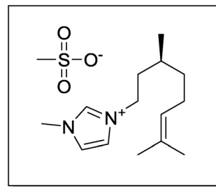
Scheme 1 Structure of the (S)-(3,7-dimethyloct-6-en-1-yl)-1-methyl-1 H -imidazol-3-ium methanesulfonate.
