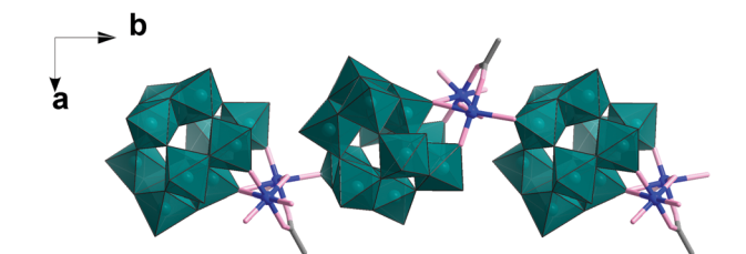
Fig. 2 Representation of the polyanion chain structure of 2 . The \{W_{11}\} building units are shown as teal polyhedra, Cu as blue ball, O and C as rose and grey sticks.
