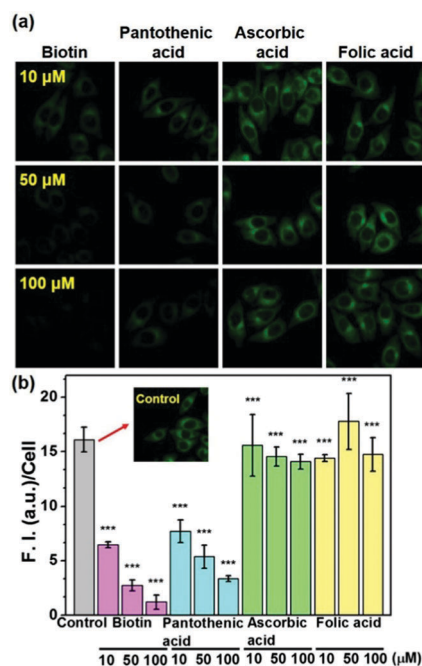
Fig. 3 (a) Effect on the uptake of 5 in HeLa cells in the presence of vitamins biotin, pantothenic acid, ascorbic acid and folic acid. The cells were incubated with 2 \mu M of the probe in presence of the vitamin under high glucose serum free DMEM media at 37 ^{\circ} C, \lambda_{\text{ex}} = 458 nm, bandpath filter (505–550 nm). (b) Fluorescence intensity (F.I.) per cell in the images of the panel (a). The images were analysed by Image J software. The data are presented as mean \pm SD ( n = 5).
