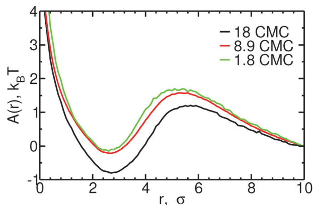
Fig. 4 Free energy, A(r) , as a function of the distance r between micelles of size n = 9\text{--}13 and monomers, for different concentrations. Curves are shifted so that A(r = 10) = 0 , for ease of viewing.
