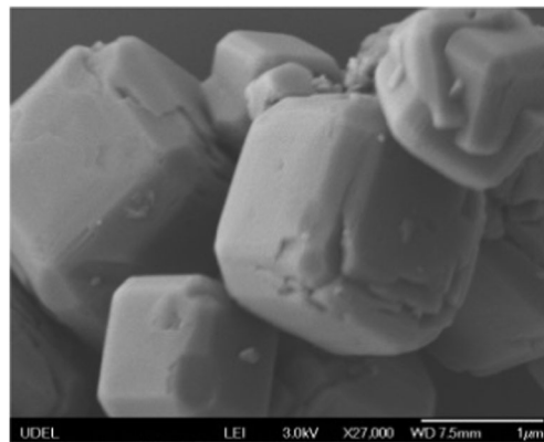
Fig. 1 SEM image of cubic aluminosilicate zeolite particles used in this study. The scale bar in the lower right is 1 µm.
