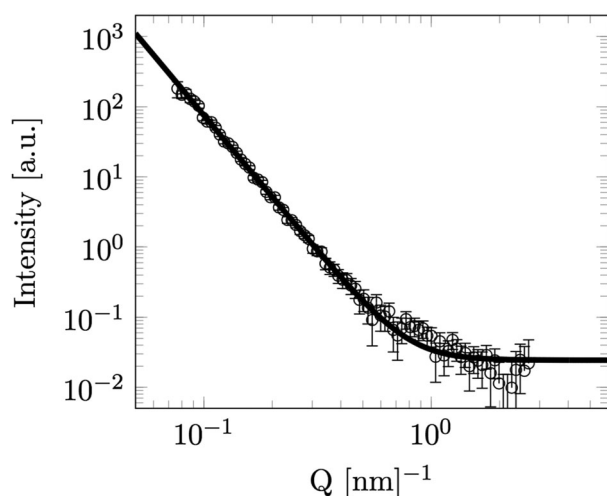
Fig. 4 SANS data for a low concentration solution of Stöber silica particles in \text{D}_2\text{O} . Line is fit to Porod scattering with a fractal index ( n ) of 3.90 \pm 0.03 .
