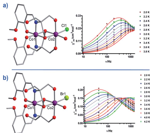
Fig. 15 Molecular structures of [\text{Co}^{\text{III}}\text{Co}^{\text{II}}(\text{LH}_2)_2\text{X}(\text{H}_2\text{O})](\text{H}_2\text{O})_4 and the frequency dependence of the out-of-phase magnetic susceptibility collected in a 1000 Oe dc field. (a) \text{X} = \text{Cl} (21) and (b) \text{X} = \text{Br} (22). Colour code: purple (Co), bright green (Cl), light green (Br), blue (N), red (O), grey (C). Hydrogen atoms omitted for clarity. Reprinted with permission from ref. 44. Copyright (2014) American Chemical Society.
