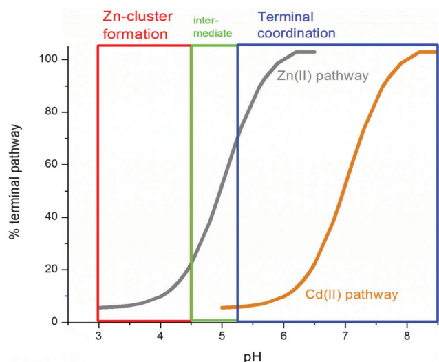
Fig. 9 Change in \text{Zn(II)} metalation pathway as a function of pH (grey line) compared to \text{Cd} (orange line). Demetalation begins to occur at \text{pH} < 4.5 so the curve was extrapolated to \text{pH} 3 based on the \text{Cd} metalation data. At the lowest physiologically relevant pH around 5.5 the binding pathway is greater than 80% terminal (blue box) and only forms clusters below \text{pH} 4.5 (red box).
