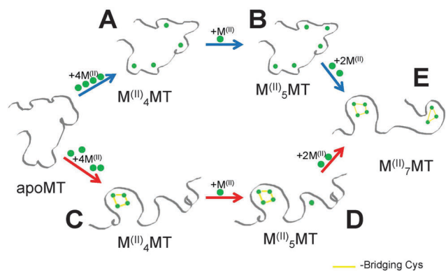
Fig. 8 Representation of the two possible pathways for metalation with \text{Zn(II)} or \text{Cd(II)} . The cooperative cluster driven pathway (red arrows) and the noncooperative beaded pathway (blue arrows). The terminally-bound, beaded structure (A) is able to coordinate an additional metal terminally, forming (B), which utilizes all twenty Cys residues, after which clusters are formed to accommodate the last two metals and form the stable two-cluster \text{M}_7\text{MT} (E). The cooperatively formed cluster (C) must coordinate additional metals in the \beta -domain (D).
