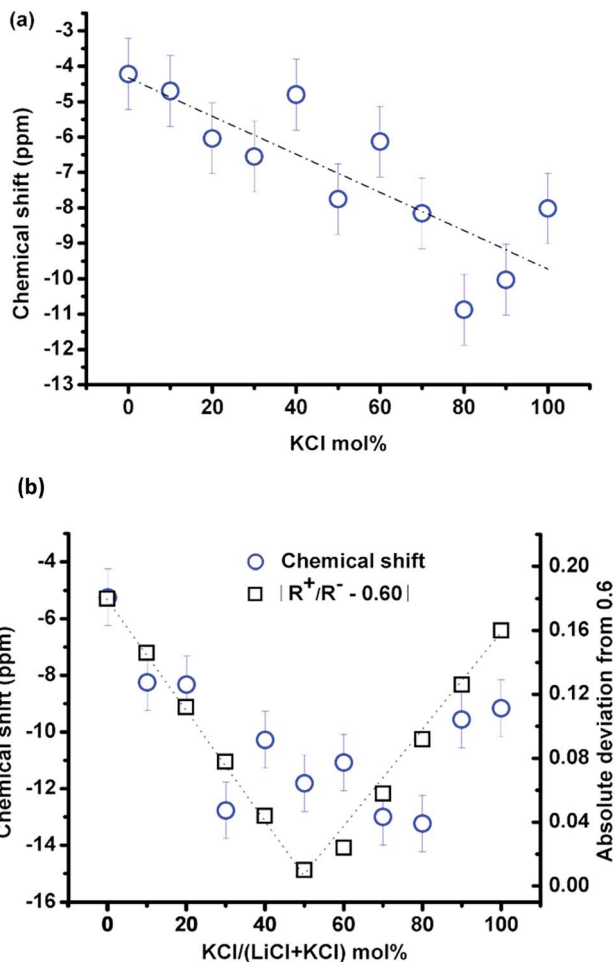
Fig. 3 (a) Variation of the ^{35}\text{Cl} chemical shifts with increasing KCl concentration in molten (Li,K)Cl at temperatures 10^\circ\text{C} above the melting point; (b) at a constant temperature of 837^\circ\text{C} (blue circles represent the chemical shift; the dotted line is a visual guide for the trend; black squares represent absolute deviation of the cation-to-anion radius ratio ( R^+/R^- ) from a critical value of 0.6, which will be discussed in detail in Section 4.1).
