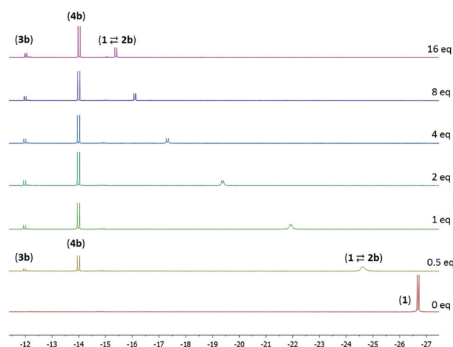
Fig. 1 Hydride region of the ^1\text{H} NMR spectrum in toluene- d_8 solvent for 1 with varying amounts of 4-pentenitrile added.
