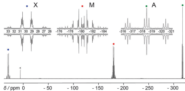
Fig. 18 ^{31}P\{^1H\} NMR spectrum of the butterfly-shaped dication 105 2+ (upwards) and simulation (downwards). This figure has been reproduced from Angewandte Chemie with permission from John Wiley and Sons. 129
