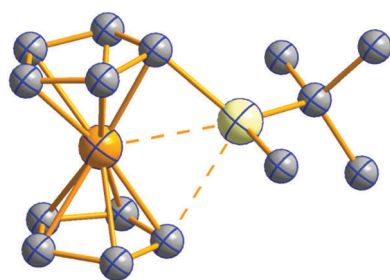
Fig. 45 Molecular structure of [\text{FcSiMe}_3\text{Bu}]^+ . K. Mütter, R. Fröhlich, C. Mück-Lichtenfeld, S. Grimme and M. Oestreich, J. Am. Chem. Soc. , 2011, 133 , 12442–12444. Data from this reference were used to draw this figure.
