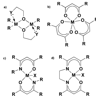
Fig. 17 Single-source precursors for gallium and indium oxide ( \text{M} = \text{Ga}, \text{In} ).
