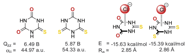
Fig. 6 Molecular structures, quadrupole moments and molecular polarizabilities of selected thio cyanuric acid derivatives and their corresponding anion- \pi complexes with chloride (including the calculated interaction energies and equilibrium distances). Additionally, the ion pairs of the ethylene ammonium-substituted chloride salts of the thio- ( 10 ) and dithiocyanuric acids ( 11 ) are shown as observed in the solid state. 19c
