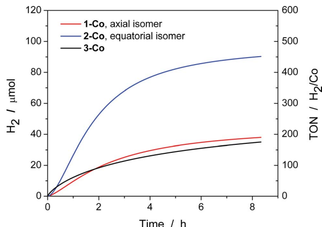
Fig. 8 Photocatalytic H_2 production of 1-Co , 2-Co , and 3-Co with [\text{Ru}(\text{bpy})_3]^{2+} and ascorbic acid under 452 \pm 10 nm (540 mW). H_2 evolution and TON vs. time measured over 8 h of photocatalysis. Conditions: 2.0 \times 10^{-5} M \text{Co(II)} catalyst, 3.3 \times 10^{-4} M [\text{Ru}(\text{bpy})_3]^{2+} , and 0.3 M \text{H}_2\text{A}/\text{HA}^- at pH 5.5.
