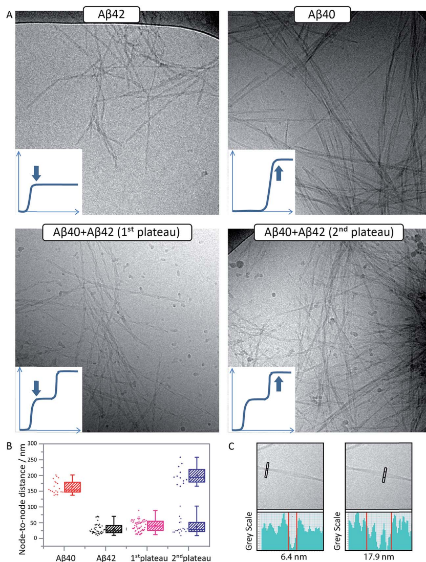
Fig. 5 A \beta 42 and A \beta 40 form distinct, separate fibrils. (A) Cryo-TEM images of pure A \beta 42 fibrils (top left), pure A \beta 40 fibrils (top right) and fibrils formed in an equimolar mixture of A \beta 42 and A \beta 40 at the 1 st (lower left) and 2 nd (lower right) plateaus are shown. Pure A \beta 42 fibrils are short and twisted with a shorter helical repeat. Pure A \beta 40 fibrils are larger, straighter and thicker. The samples contain 5 \mu M ThT, 20 mM sodium phosphate, 200 \mu M EDTA, 0.02% NaN 3 , pH 7.4. (B) An analysis of the node-to-node distance yields a quantitative measure for the two morphologies confirming that fibrils collected at the 1 st plateau have similar morphology as A \beta 42 fibrils, while the fibrils collected at the 2 nd plateau display both types of morphologies. Points show individual measurements. The box contains the middle 50%, the line indicates the median, and the whiskers include all data points. (C) Zoom-ins of pure A \beta 40 fibrils illustrating the method used for finding the nodes for node-to-node distance measurements. The nodes were defined as points along the fibril where a single minimum gray scale was observed (left), while between the nodes several minima are observed which is due to multiple protofilaments involved in the same fibril (right).
