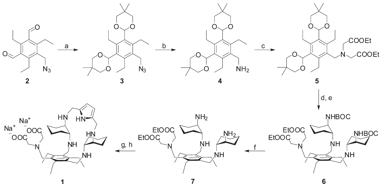
Scheme 1 Synthesis of receptor 1 . Reagents and conditions: (a) neopentylglycol, p -TsOH cat., toluene, reflux, overnight, 87%; (b) \text{LiAlH}_4 , THF, r.t., 2.5 h, 92%; (c) ethyl bromoacetate, \text{KHCO}_3 , DMF, r.t. overnight, 83%; (d) \text{HCl} 1 M, THF, overnight; (e) N -BOC-(1 R , 2 R )-1,2- trans -diaminocyclohexane, \text{CHCl}_3 , reflux, overnight, then \text{NaBH}_4 suspension in MeOH, r.t., 1 h, 62%; (f) TFA, \text{CH}_2\text{Cl}_2 , r.t., 2 h, 79%; (g) pyrrole-2,5-dicarbaldehyde, \text{CHCl}_3 , r.t., then \text{NaBH}_4 suspension in MeOH, r.t., 1 h, 70%; (h) \text{NaOH} , \text{H}_2\text{O}/\text{EtOH} 1:1, r.t., overnight, 81%.
