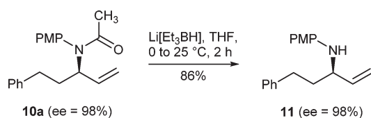
Scheme 3 Reductive acetamide cleavage.
