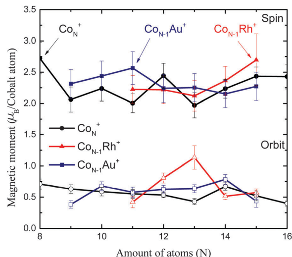
Fig. 4 The Langevin scaled spin (full symbols) and orbital (empty symbols) magnetic moments of \text{Co}_n\text{Rh}^+ (red triangles) and \text{Co}_n\text{Au}^+ (blue squares), assuming n_h = 2.5 . Also plotted are the results obtained for pure cobalt clusters obtained by Peredkov et al. 4 using the same setup as this work (black circles).
