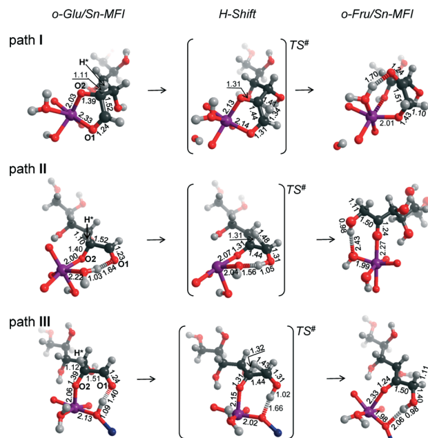
Fig. 7 Local structures of reaction intermediates and transition states for the aldose-ketose isomerization of o -Glu over the SnOH site in a periodic Sn-MFI model.
