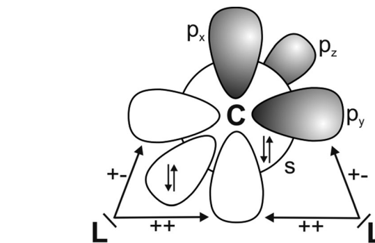
Fig. 1 Schematic presentation of the orbital interactions between carbon atom in the ( 1s^2 2s^2 2p_x^0 2p_y^0 2p_z^2 ) ^1D state and two \sigma donor ligands L. The ++ sign indicates the in-phase combination of the donor orbitals into the vacant 2p_x orbital ( \sigma symmetry) while the +,− sign denotes the out-of-phase combination of the donor orbitals into the vacant 2p_y orbital (in-plane \pi_{\parallel} symmetry).
