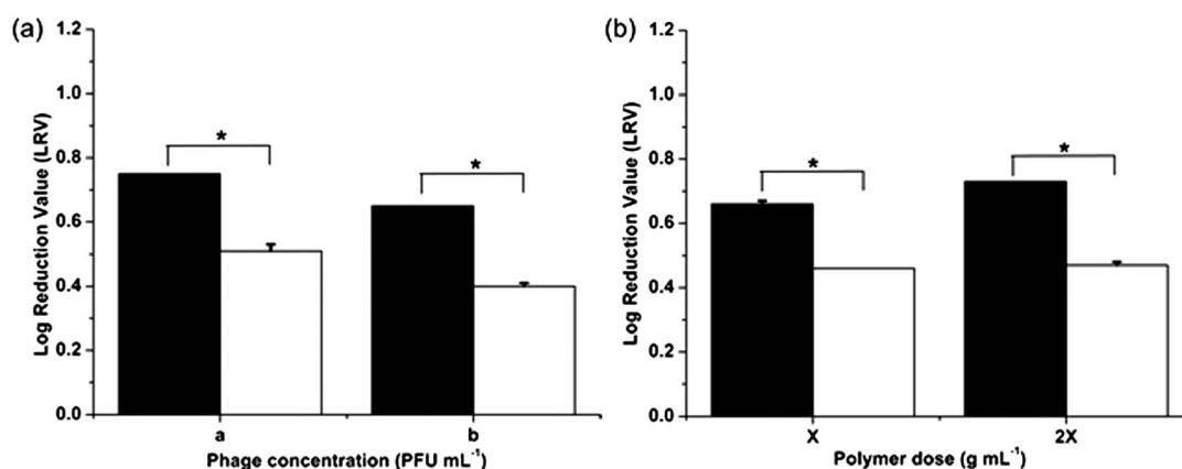
Fig. 3 Virucidal effect of nanoparticles on phage viability at different (a) phage concentrations; a: 6300 \text{ pfu mL}^{-1} ; b: 63000 \text{ pfu mL}^{-1} and (b) polymer doses; X: 0.005 \text{ g mL}^{-1} . Statistical significance was denoted by *. Student's t -test: p < 0.01 (■ – \text{vMIP}_{\text{MAA}} ; □ – \text{NIP}_{\text{MAA}} ).
