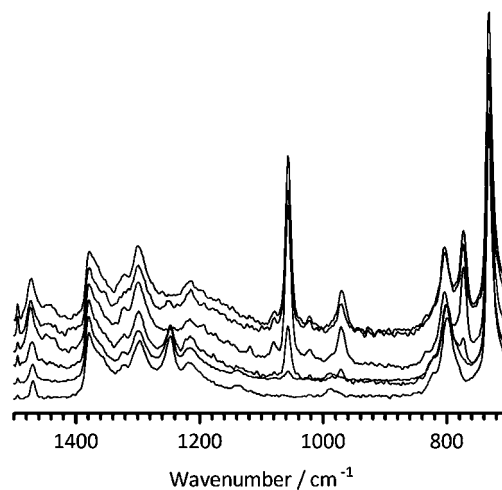
Fig. 1 The FT-Raman spectra (diagnostic region 1500–700 cm -1 ) of the Nafion-DMP(F - ) membranes formed on the reaction of Nafion-SO 2 F and 14DMP at room temperature for (from bottom to top): 0 h (i.e. pristine Nafion-SO 2 F ), 3 h, 24 h, 100 h, 144 h, and 196 h. Spectra were normalised to the band at 1380 cm -1 and then stacked for clarity of presentation.
