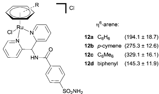
Fig. 7 A series of piano-stool Ru(II) arene CA inhibitors with inhibition constants (nM, K_{\text{S}} ) in parenthesis (hCA II).
