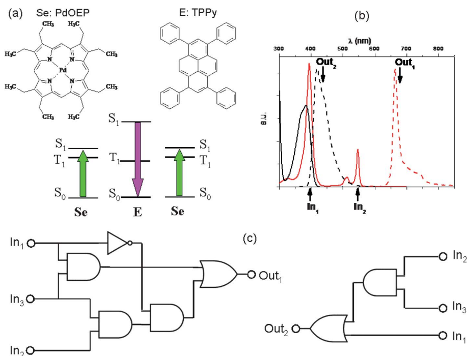
Fig. 7 A TA up-conversion process involving PdOEP as sensitizer (Se) and TPPy as emitter (E), whose molecular structures are in (a) along with a scheme of their relative energy levels. The pair PdOEP–TPPy convert green light into violet light. In (b) the continuous traces represent the absorption spectra (in black that of TPPy and in red that of PdOEP), whereas the dashed traces represent the emission spectra (black for TPPy and red for PdOEP). (c) If we choose \lambda_{\text{exc}} = 400 \text{ nm} , \lambda_{\text{exc}} = 546 \text{ nm} and \text{N}_2 as the first ( \text{In}_1 ), second ( \text{In}_2 ) and third ( \text{In}_3 ) inputs, respectively, complicated binary logic circuits can be implemented with the phosphorescence of PdOEP ( \text{Out}_1 ) and the fluorescence signal of TPPy ( \text{Out}_2 ) as outputs.
