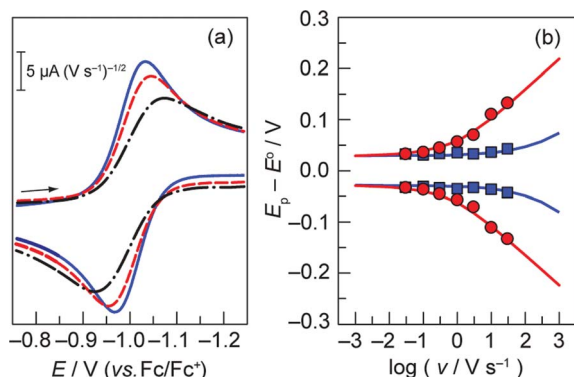
Fig. 1 (a) Overlay of representative normalized ( i_{\text{norm}} = i/v^{1/2} ) ( i is current, v is scan rate) CVs taken of a 0.3 mM solution of cobalt porphyrin 3 in acetonitrile with 0.03 (—•), 0.3 (—•), and 3 (—•) \text{V s}^{-1} scan rates, using a glassy carbon electrode. (b) Difference between anodic or cathodic peak potential and midpoint potential ( E_p - E^0 ) vs. \log of scan rate ( E^0 = -1.00 V for the \text{Co}^{2+/+} couple (●), and -1.98 V for the \text{Co}^{+/0} couple (■)). Simulated curves are plotted for k_s = 0.011 \text{cm s}^{-1} (—) and k_s = 0.2 \text{cm s}^{-1} (—). The diffusion coefficient ( D ) of 3 was determined to be 8 \times 10^{-6} \text{cm}^2 \text{s}^{-1} from the peak current, i , in the reversible limit: i = 0.446FAc^0D^{1/2}(Fv/RT)^{1/2} ( F is the faraday constant, A is the area of the electrode and C^0 is the bulk porphyrin concentration).
