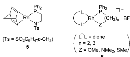
Chart 2 The Rh catalysts bearing P-L type bidentate ligands.
