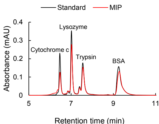
Fig. 7 The chromatogram of standard protein mixture with 0.018 mM of each protein (black line) and protein mixture after the adsorption with MIP hydrogel (red line).
