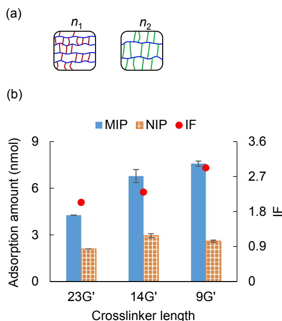
Fig. 3 (a) A illustration of the polymer network when the crosslinker length changed. Here, n_1 < n_2 , i.e. the left illustration represents the shorter crosslinker polymer network, the right one represents the longer crosslinker polymer network. (b) The adsorption amount and imprinting factor (IF) of the gels fabricated with different crosslinkers.
