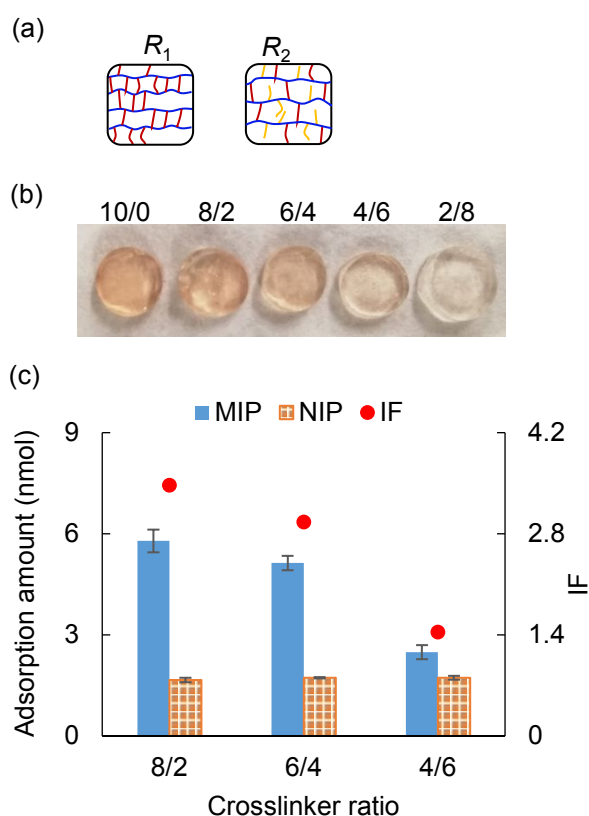
Fig. 4 (a) A illustration of the polymer network when the crosslinker ratio changed. Here, R_1 > R_2 , i.e. the left illustration represents the dense crosslinked polymer network, the right one represents the light crosslinked polymer network. (b) The picture of MIP hydrogels with different crosslinker ratios after a 24 h washing in 1 M NaCl at room temperature. (c) The adsorption amount and imprinting factor (IF) of the gels with different crosslinker ratios of PEGDA/PEGA.
