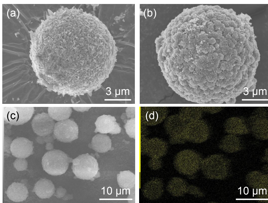
Fig. 5 (a) High-magnification SEM images of ZIF-8/HSMC-SB Hmim and (b) ZIF-8/HSMC-SB Zn , (c) low-magnification SEM image, and (d) EDS mapping of Zn for ZIF-8/HSMC-SB Zn .
