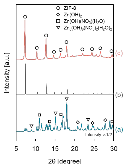
Fig. 4 XRD patterns of the ZIF-8/HSMC-SB prepared by the semi-batch operation. (a) ZIF-8/HSMC-SB Hmim prepared by feeding the Hmim aqueous solution into the \text{Zn}^{2+} aqueous solution, (b) simulated ZIF-8, and (c) ZIF-8/HSMC-SB Zn prepared by supplying the \text{Zn}^{2+} aqueous solution into the Hmim aqueous solution.
