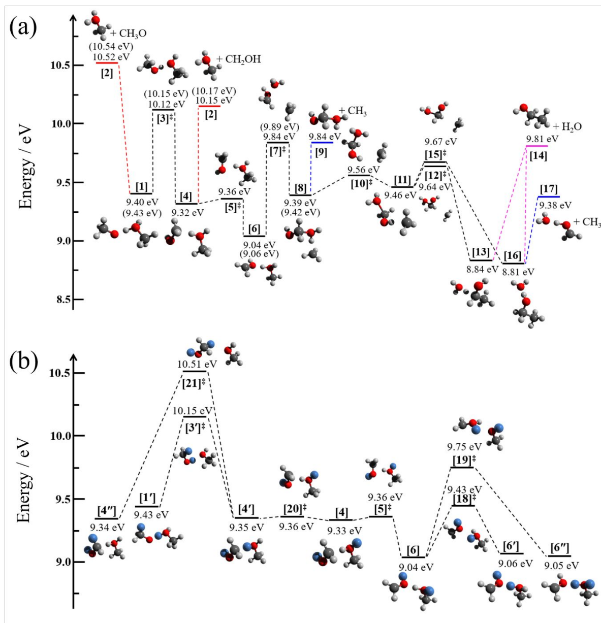
Figure 3. (a) Fragmentation pathways of the light methanol dimer cation to produce the fragment ions m/z 33, 46, and 49 by hydroxymethyl, water, and methyl loss, respectively. The G4-computed energies are given with respect to the neutral dimer. The energy thresholds for the perdeuterated dimer cation are given in parentheses. (b) Hydrogen scrambling mechanism in the dimer cation shown with the help of the (\text{CH}_3\text{OD})_2^+ dimer cation.
