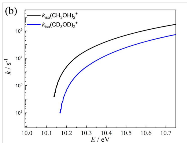
Figure 4. (a) Statistical model of the dissociative ionization of the methanol and the perdeuterated methanol dimer. Open circles and stars represent the experimental fractional abundances in the methanol dimer and perdeuterated methanol dimer experiments, respectively. The solid and dashed lines show the simulated methanol dimer and perdeuterated methanol dimer breakdown curves, respectively. (b) Isomerization rate constant of (\text{CH}_3\text{OH})_2^+ and (\text{CD}_3\text{OD})_2^+ over [\mathbf{3}]^\ddagger in the statistical model as a function of energy relative to the neutral.
