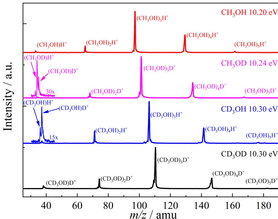
Figure 2. Threshold photoionization mass spectra of light, selectively deuterated and perdeuterated methanol clusters at representative photon energies.
