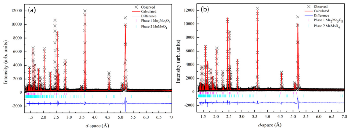
Fig. 2 Rietveld refinement of the X-ray diffraction data collected for \text{Mn}_2\text{Mo}_3\text{O}_8 and fitted to the P6_3mc model 47 at (a) 298 K ( wRp = 7.5\% , R_p = 5.74 , \chi^2 = 2.7 ) and (b) 12 K ( wRp = 8.6\% , R_p = 6.3\% , \chi^2 = 3.5 ). Black crosses represent observed data, red line represents the calculated model and the blue line represents the difference between the observed and calculated data. \text{Mn}_2\text{Mo}_3\text{O}_8 is represented by the magenta tick marks (top) and \text{MnMoO}_4 by the cyan tick marks (bottom).
