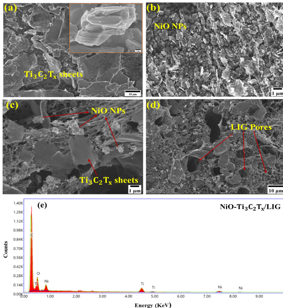
Fig. 2 FESEM images of (a) \text{Ti}_3\text{C}_2\text{T}_x MXene flakes, (b) NiO nanoparticles and (c) and (d) the \text{NiO}-\text{Ti}_3\text{C}_2\text{T}_x/\text{LIG} composite at different magnifications. (e) EDS elemental spectra of the \text{NiO}-\text{Ti}_3\text{C}_2\text{T}_x/\text{LIG} nanocomposite.
