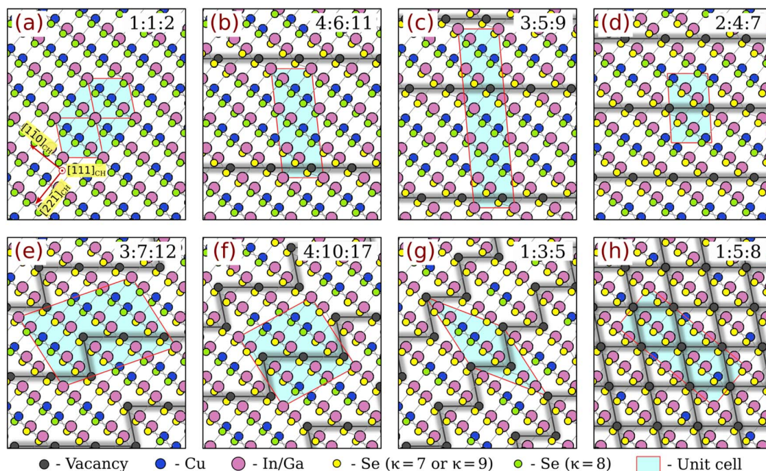
Fig. 5 Crystal structures of eight selected (near-)stable structures from the toptotactic series. The black lines connect vacancies separated by a (i.e. lattice parameter of the zinc-blende conventional cell) and the shaded grey regions are included to help visualize the vacancy arrangements.
